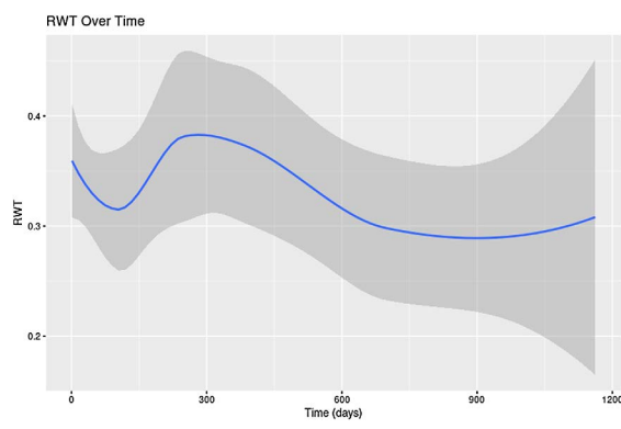
Figure 2. LOESS curves of RWT over time, beginning on the day of baseline echocardiogram prior to anthracycline therapy, and continuing throughout therapy and until at least 1 year after therapy.
