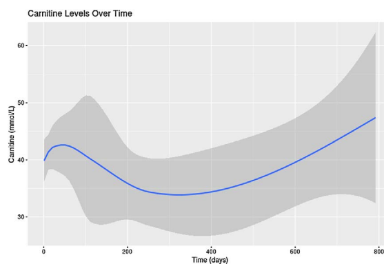
Figure 3. LOESS curves of serum carnitine concentrations over time, beginning on the day of baseline echocardiogram prior to anthracycline therapy, and continuing throughout therapy and until at least 1 year after therapy.
